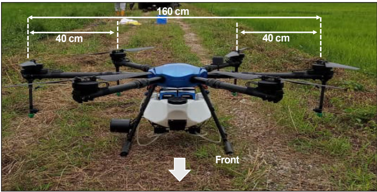
Figure 2. Drone configuration with four nozzles beneath each rear rotor, spaced 40 cm apart
